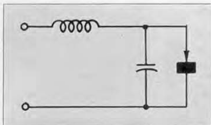
FIGURE 3. Diagram showing the resonant circuit formed by lead inductance and shunt capacitance of a crystal rectifier.
