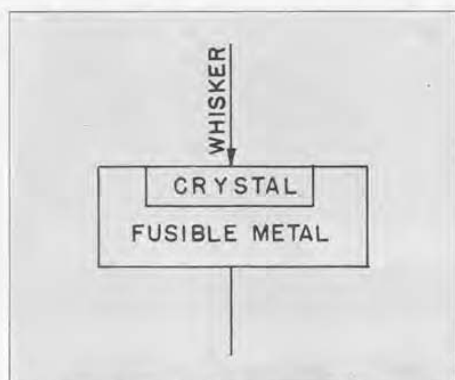
FIGURE 2. Simplified diagram of the construction of a crystal rectifier.
