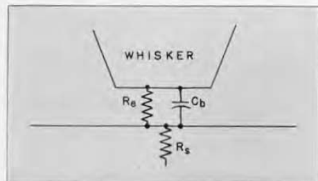
FIGURE 6. Simplified sketch of the whisker-crystal contact greatly enlarged to show the location of the elements of Figure 5.
